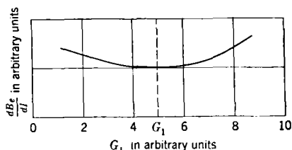
FIG. 10-6.— (dB_e/dI) as a function of G_L .
